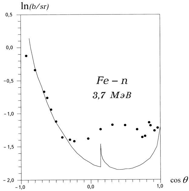
Figure 2: Classical scattering of nonrelativistic neutrons with energy 3,7 Mev on nuclei of iron
