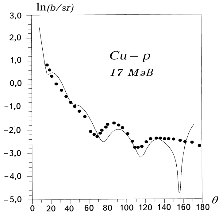
Figure 3: Elastic scattering of protons with energy 17 Mev on the copper nuclei
