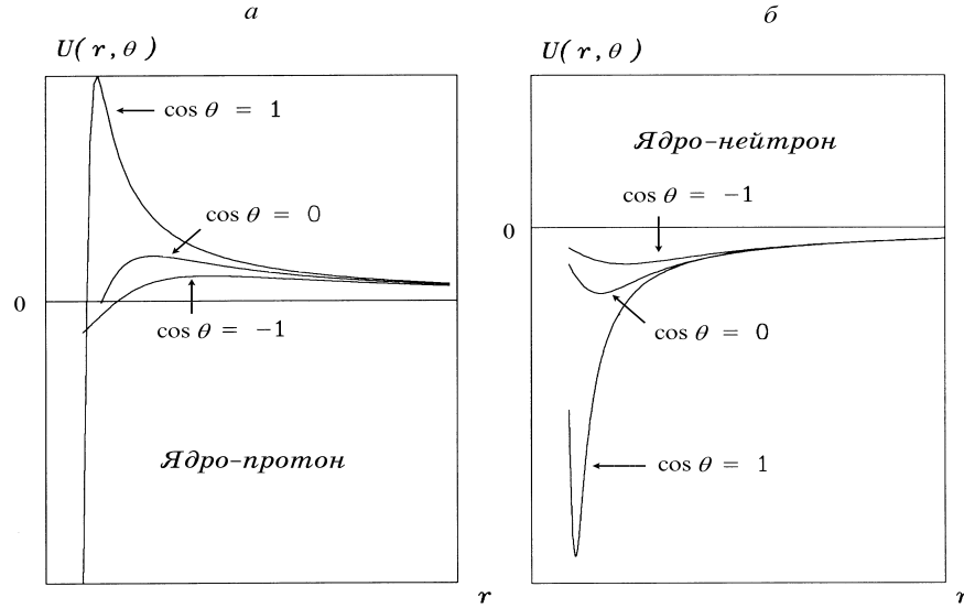
Figure 1: The drawings of potential energy dependence from spin orientation: a - potential energy of protons scattering on polarized target with r_e/r_N = -2 , r_N/r_s = 1,5 ; b - the same for neutrons with r_e/r_N = 0 , r_N/r_s = 1,5
